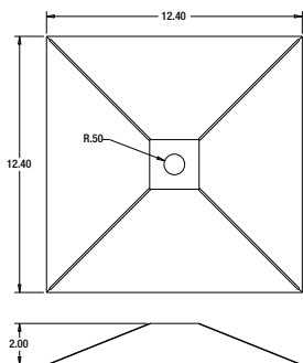
Accessory: Bird Guard
