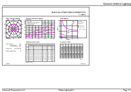
LEDBulb 6-40W A19 E26 450lm CL
