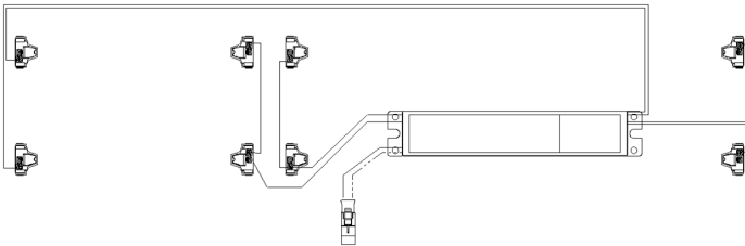
8' - 4 lamp with dual ended AC
