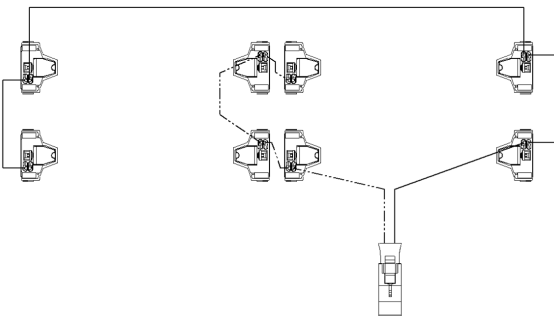
8' - 4 lamp with dual ended AC
