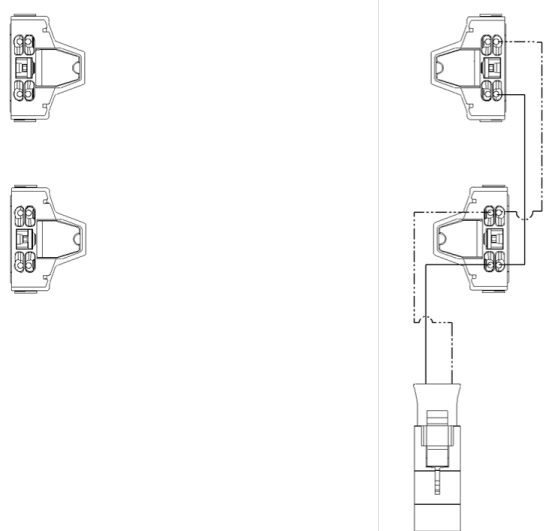
4' - 2 lamp with single ended AC
