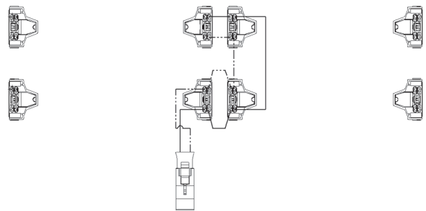
8' - 4 lamp with single ended AC
