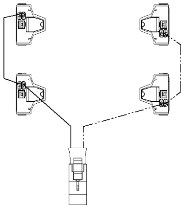
4' - 2 lamp with dual ended AC
